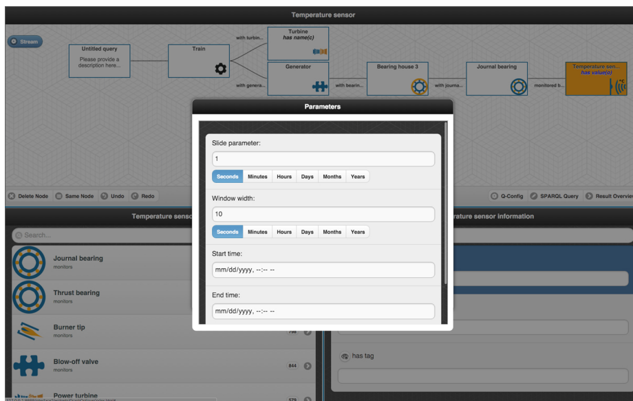
Fig. 2. OptiqueVQS with stream querying – parameter selection.
